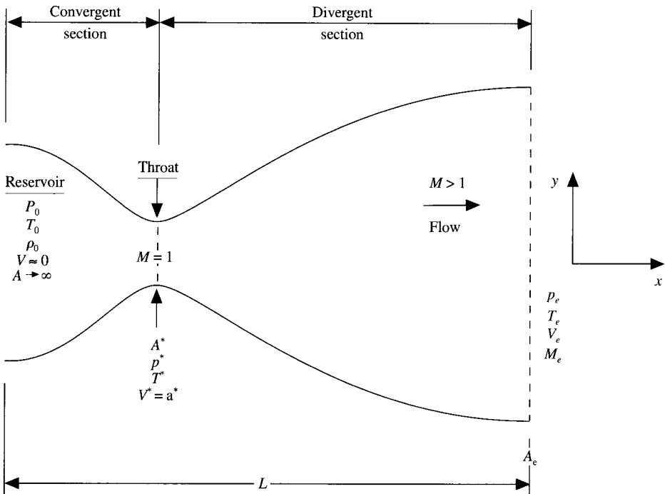
FIG. 7.1 Schematic for subsonic-supersonic isentropic nozzle flow.
