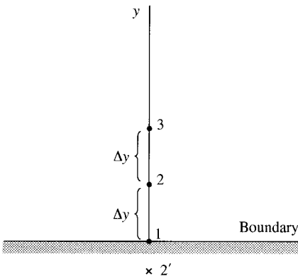
FIG. 4.4 Grid points at a boundary
