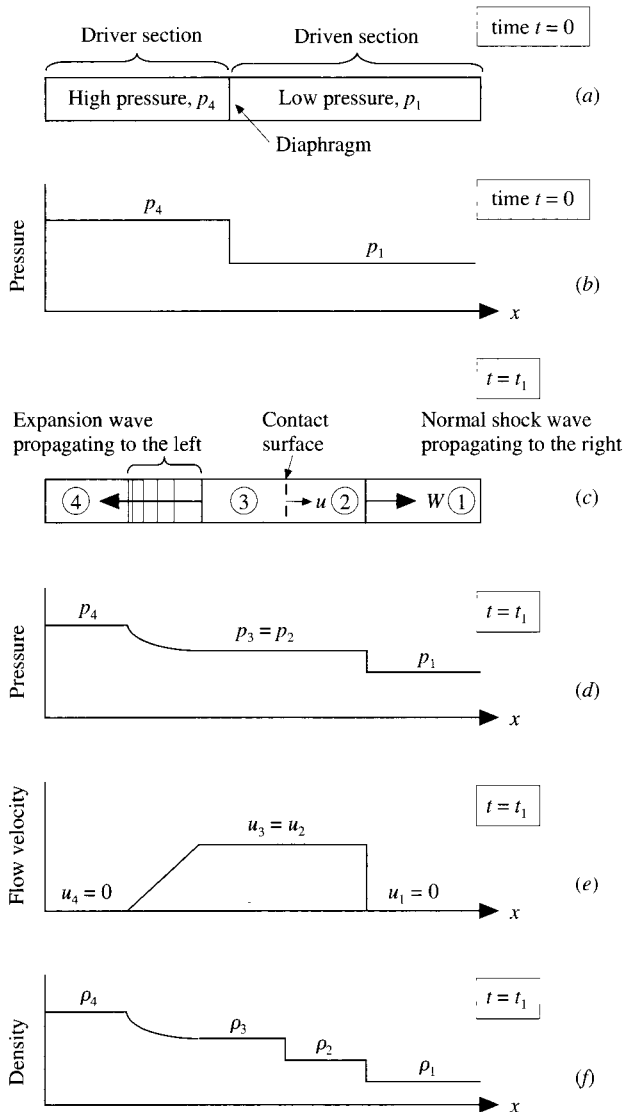
FIG. 11.5 Schematic of flow in a shock tube.
