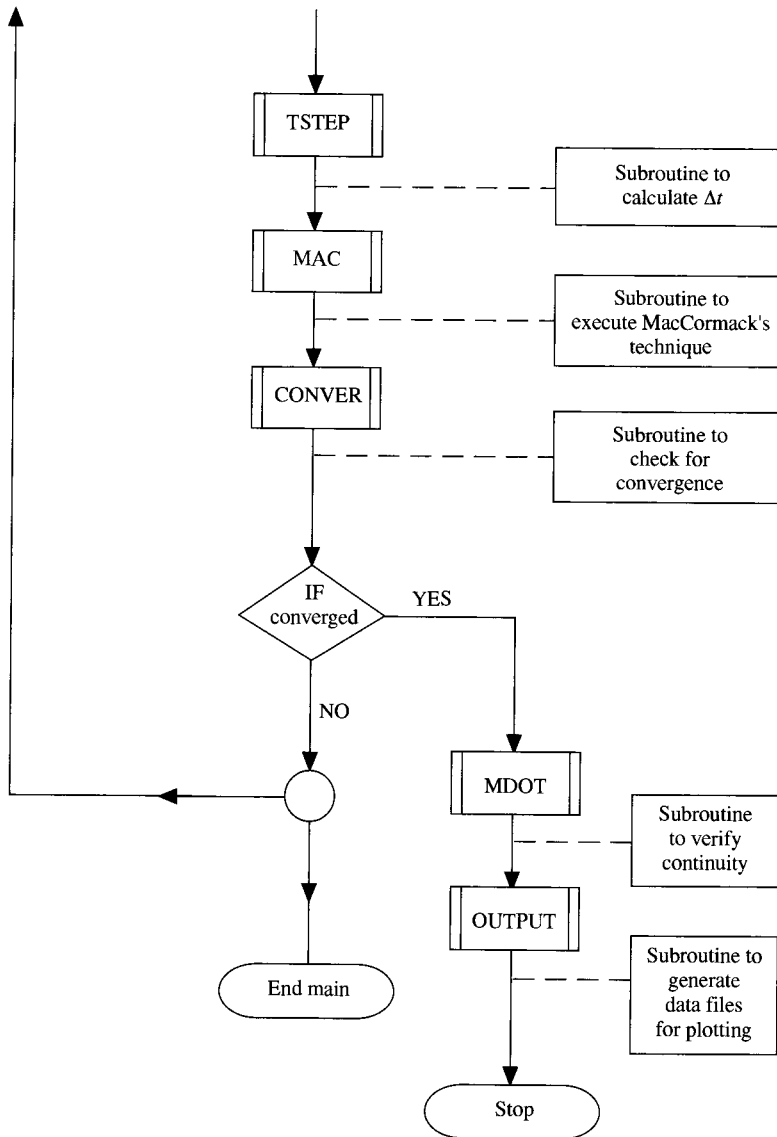
FIG. 10.7 Flowchart for the main program (MAIN).
