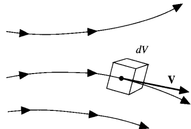
Infinitesimal fluid element moving along a streamline with the velocity \mathbf{V} equal to the local flow velocity at each point
