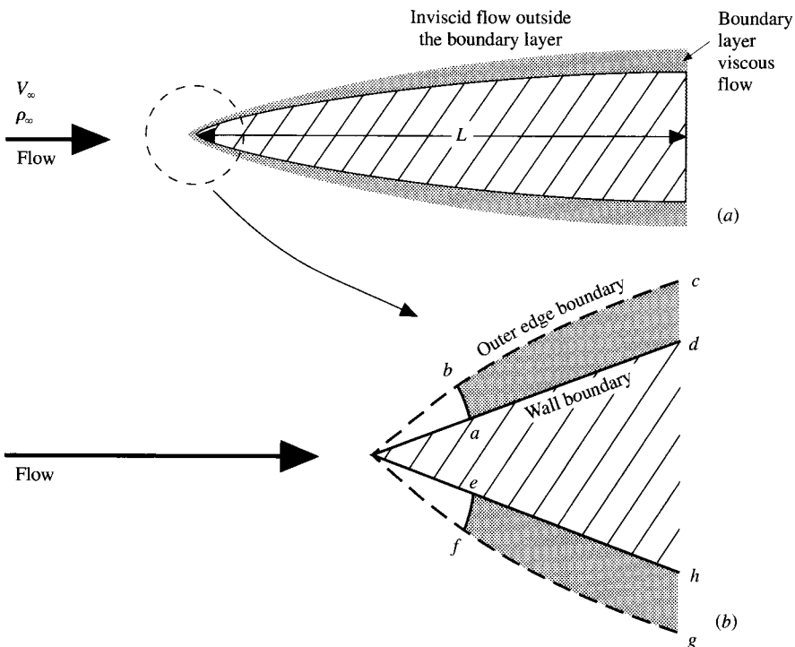
FIG. 3.10 Schematic of a boundary-layer flow.
