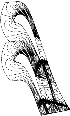
FIG. 12.8 Mach number contours around two adjacent turbine blades in an axial flow jet engine. (From Ref. 52. Reprinted with permission from Elsevier Science Publishers, Amsterdam.)
