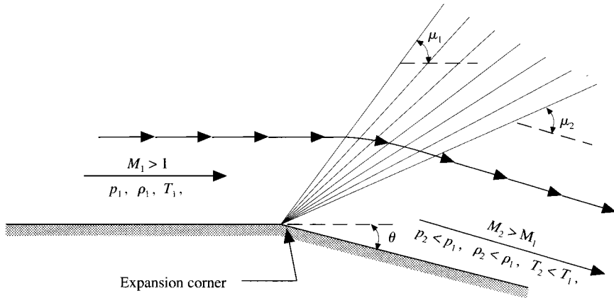
FIG. 8.1 Centered Prandtl-Meyer expansion wave.
