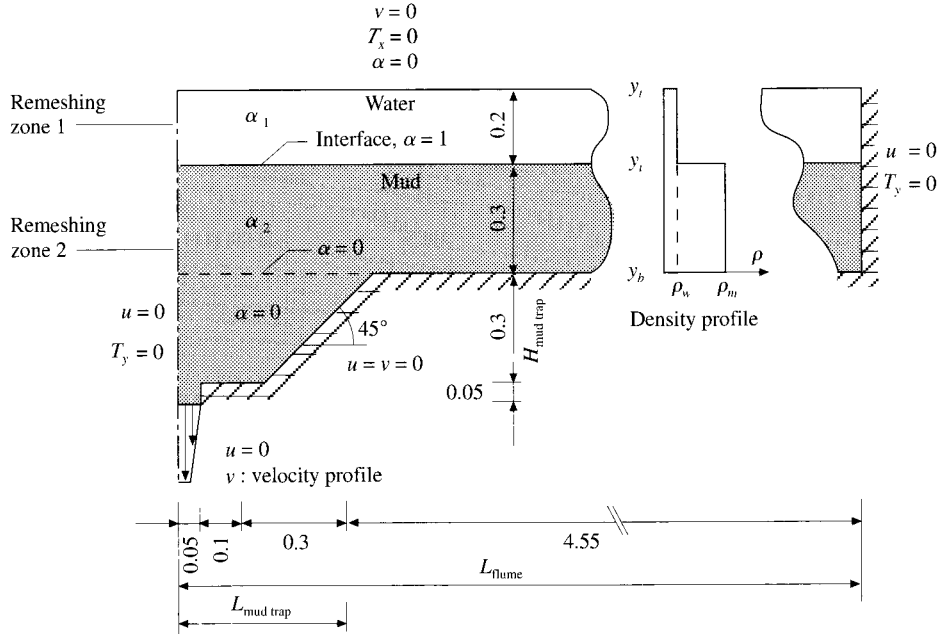
Mud and water layers in a model of a mud trap, with mud being suctioned away at the bottom left. ( After Ref. 63. )
