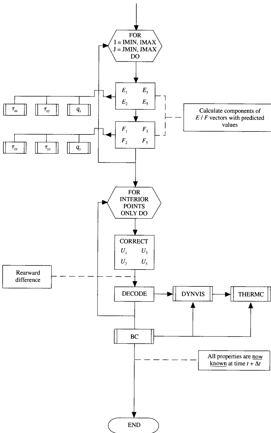
FIG. 10.8 Flowchart for MacCormack's (MAC) subroutine.
