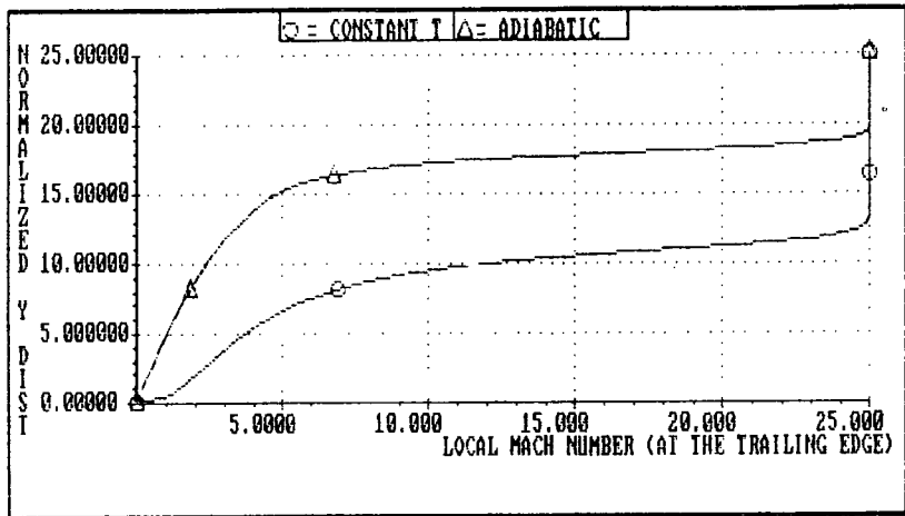
FIG. 10.17 Mach 25 at 200,000 ft; local Mach number profiles at the trailing edge.
