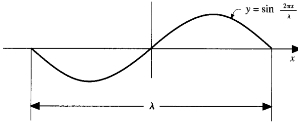
FIG. 4.10 Sine function.
