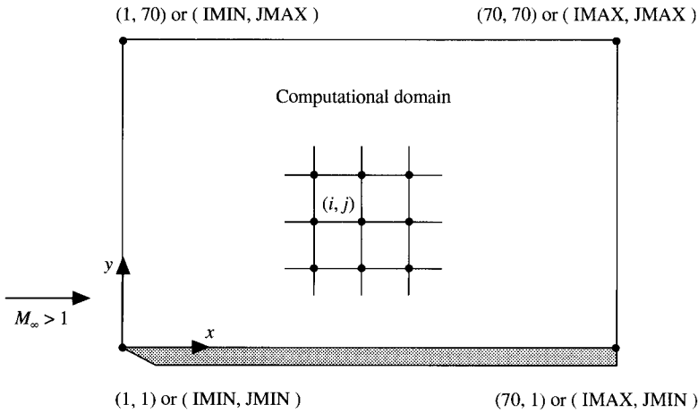
FIG. 10.3 Computational domain.
