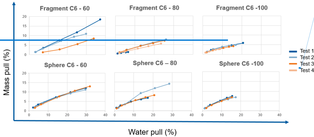
Appendix 2 Mass pull VS Water pull diagram— Fragment C6 & Sphere C6 (Medium hydrophobic)-at 60/80/100-cm column
