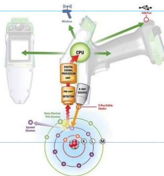
Figure 20 Schematic configuration of hand-held XRF analyzer (32)
