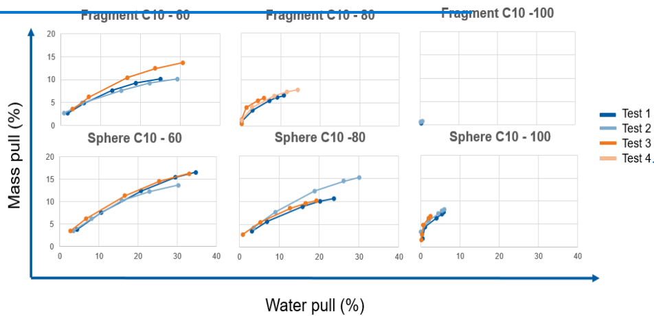
Appendix 4 Mass pull VS Water pull diagram— Fragment C10 & Sphere C10 (High hydrophobic)-at 60/80/100-cm column
