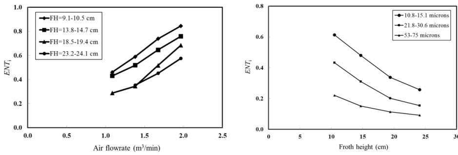
Figure 1040 Left: Effect of gas flowrate on degree of entrainment ( x > 5.3 \mu\text{m} ) at different froth height, Right: The degree of entrainment.
