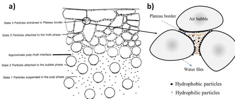
Figure 7 Recovery of the minerals during flotation process a) Location of Particles in a Flotation System (18)(17)(17) b) Froth lamella (19)(18)
