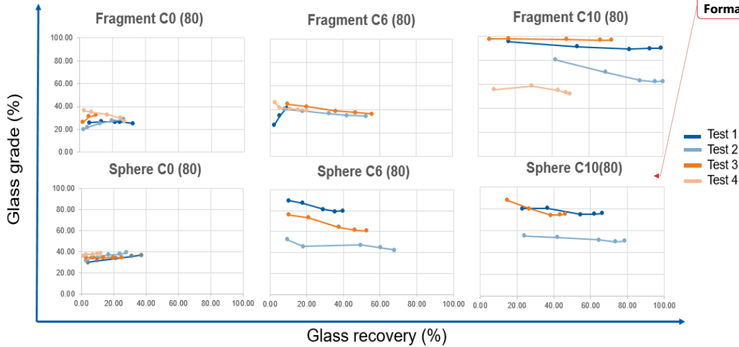
Appendix 22 HALBICH diagram – at 80 column
