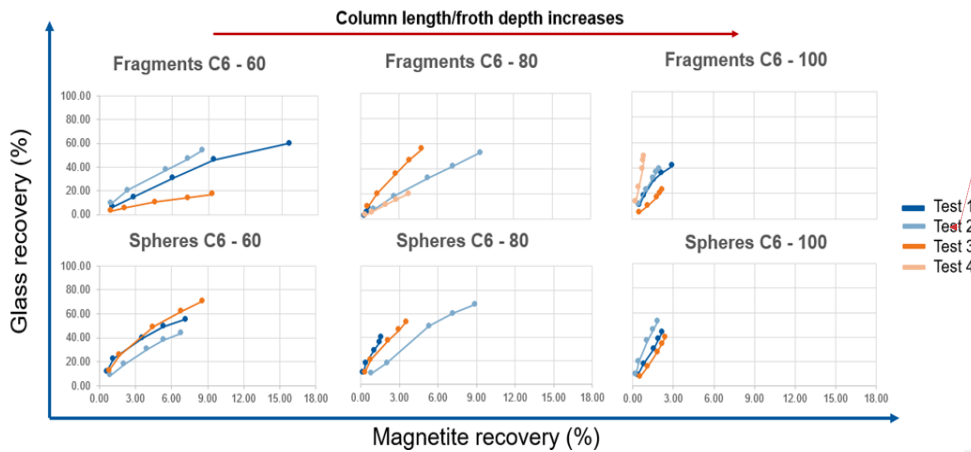
Figure 25 Fuesrstenau upgrading curve of flotation test (Test 1 – 4) in SphC6 and FragC6 at 60/80/100
