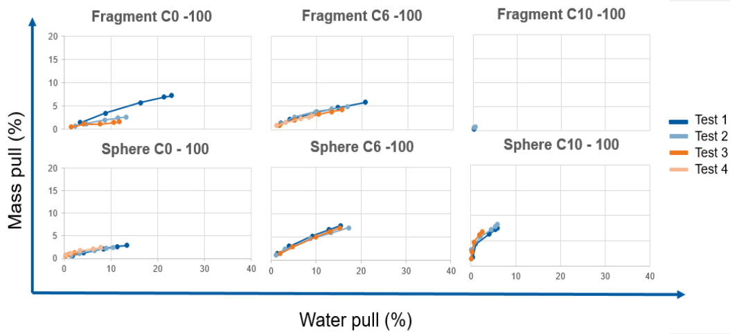
Appendix 17 Mass VS Water pull diagram Fragment and Spheres at 100cm column
