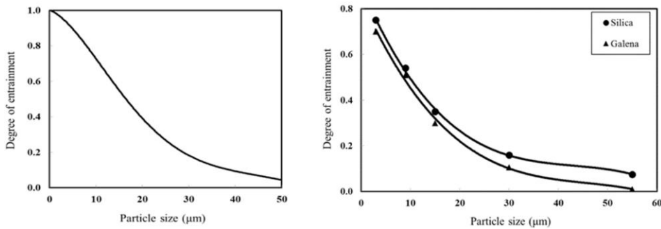
Figure 99. Left: Relationship between degree of entrainment and particle size for hydrophilic silica. Right: Effect of particle density of entrainment, silica (SG=2.6) and galena (SG=7.5) in laboratory column (20)(19)
