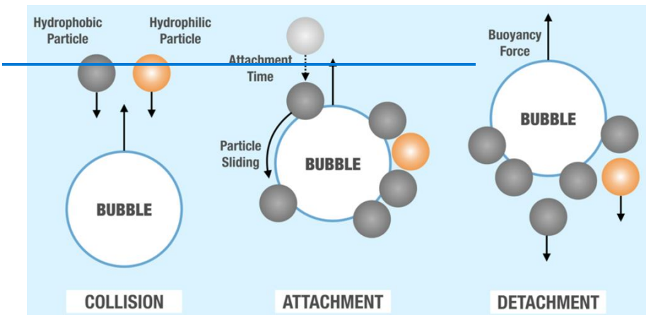
Figure 1 Flotation process procedure
