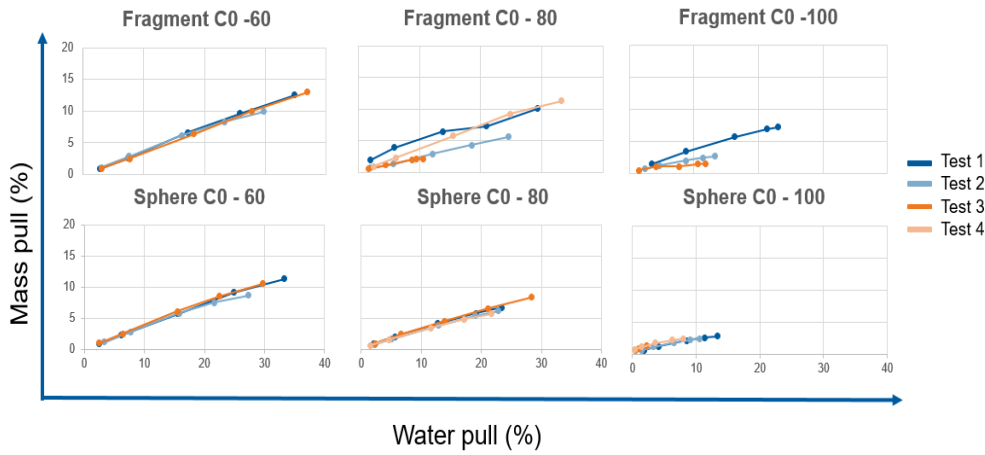
Appendix 1 Mass VS Water pull diagram – FragC0 and SphC0 (Test 1-4) at 60/80/100 cm columns
