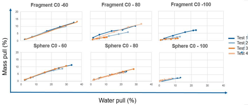
Appendix 1 Mass pull VS Water pull diagram – Fragment C0 & Sphere C0 (Hydrophilic) at 60/80/100 cm column
