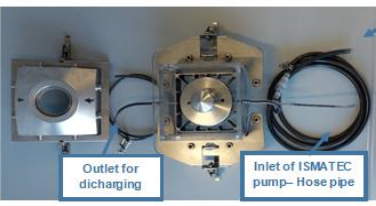
Magotteaux cell with rotor stator
