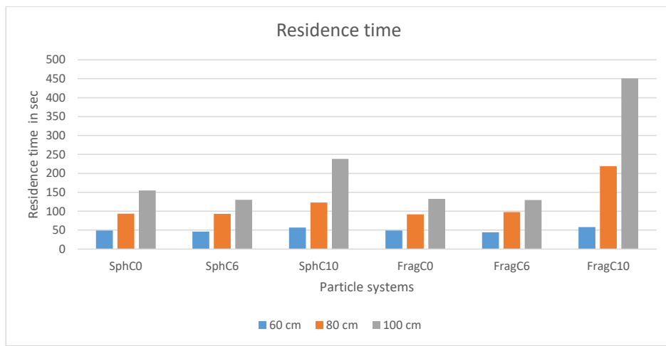
Appendix 12 Recorded froth rise residence-time in different particle systems at different column height (60/80/100).
