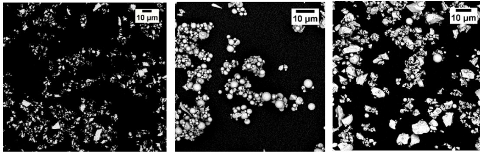
Figure 12 SEM images of the used particles system: magnetite, glass spheres, glass fragments (from left to right) (27)(26)
