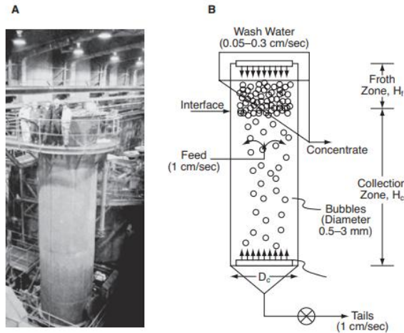
Figure 34 General schematic of conventional flotation column cell (3)
