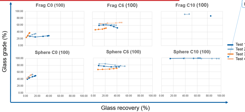
Appendix Halbich diagram – Grade and recovery of FragC10 and SphC10 particles at 60/80/10 cm columns (Test 1-4)
