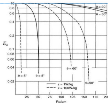
Figure 6 Relation between Stability efficiency ( E_s ) and particle size at different values of contact angle (13)
