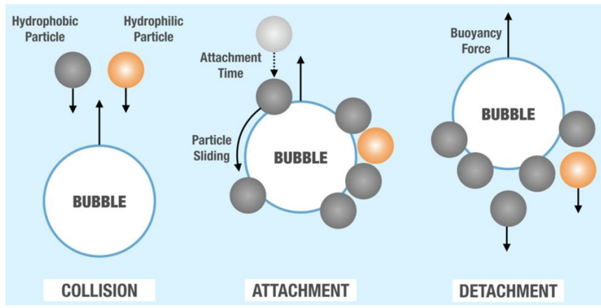
Figure 5 Flotation process (12) procedure
