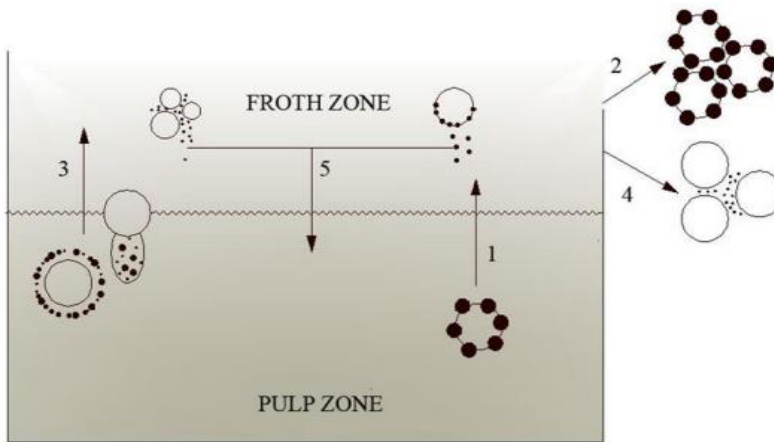
Figure 88 Mechanisms of transfer of fully liberated mineral particles in a flotation cell (20)(19)
