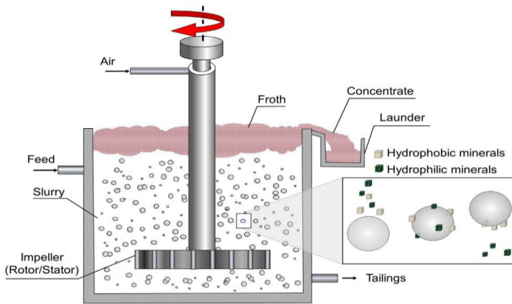
Figure 23 Principle of true flotation in a mechanical flotation cell (6)
