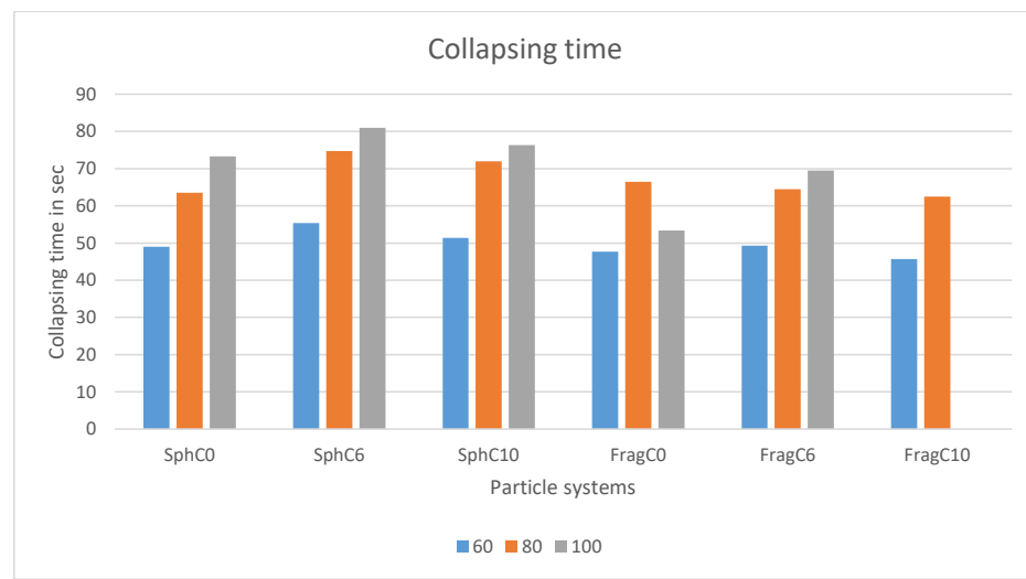
Appendix 13 Recorded collapsing time in different particle systems at different column height (60/80/100).
