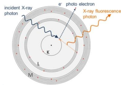
Figure 13 Sketch the X-Ray fluorescence (XRF) process (19)
