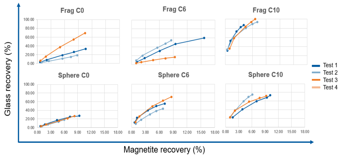
Appendix 18 Fuesrstenau upgrading curve of flotation test at 60 cm column
