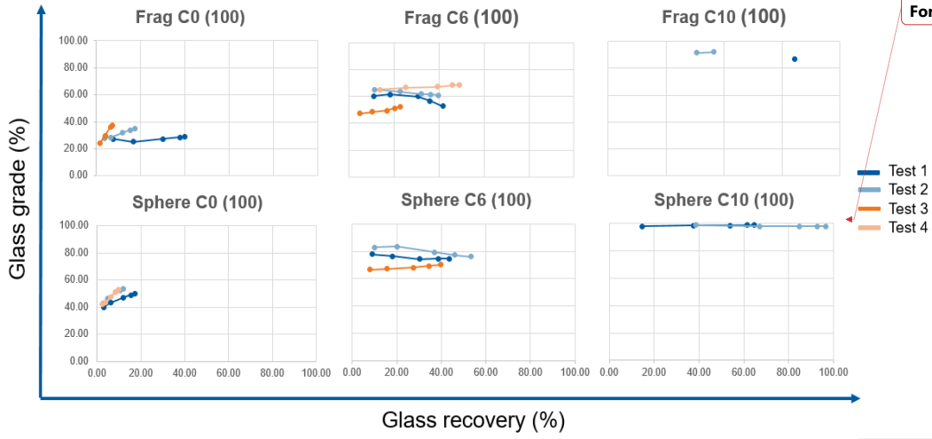
Appendix 23 HALBICH diagram – at 100 column
